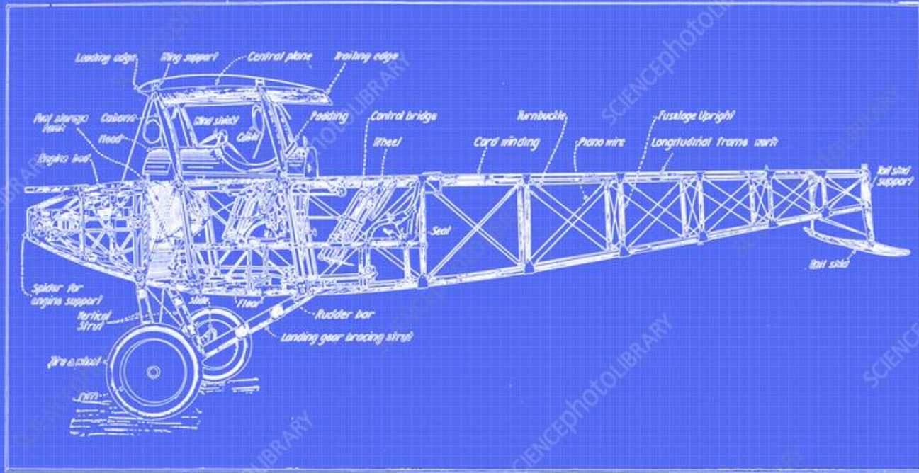
General view of an airplane with fuselage covering removed, showing details of body construction
